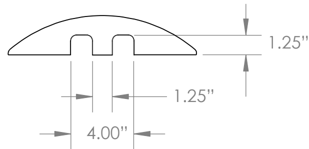
Channels End View
